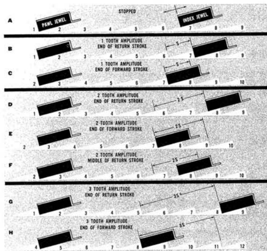
Fig. 13 Diagram of Indexing Mechanism Operation
