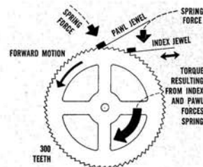
Fig. 12 Diagram of Indexing Mechanism
