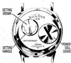
Fig. 1 Rear View of ACCUTRON Case
