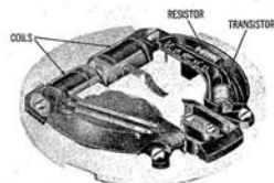
Fig. 10 Tuning Fork and Associated Circuit Elements (Front View)
