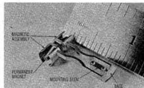
Fig. 9 ACCUTRON Tuning Fork
