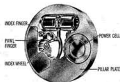
Fig. 11 ACCUTRON Indexing Mechanism (Rear View)
