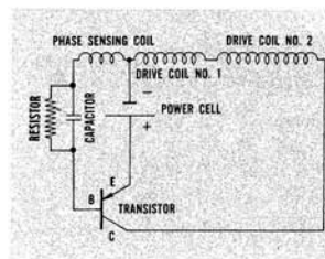
Fig. 15 Schematic Diagram of ACCUTRON Circuit
