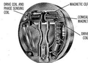
Fig. 14 Cutaway View of ACCUTRON Electro-magnetic Elements
